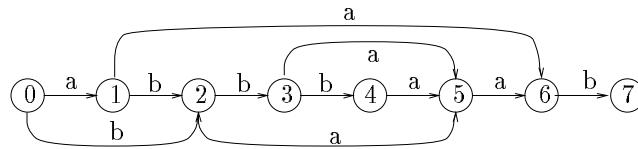
Figure2. Factor oracle of abbbaab . The word aba is recognized whereas it is not a factor.
