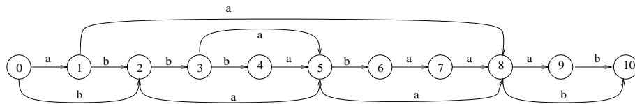
(a) Factor oracle
