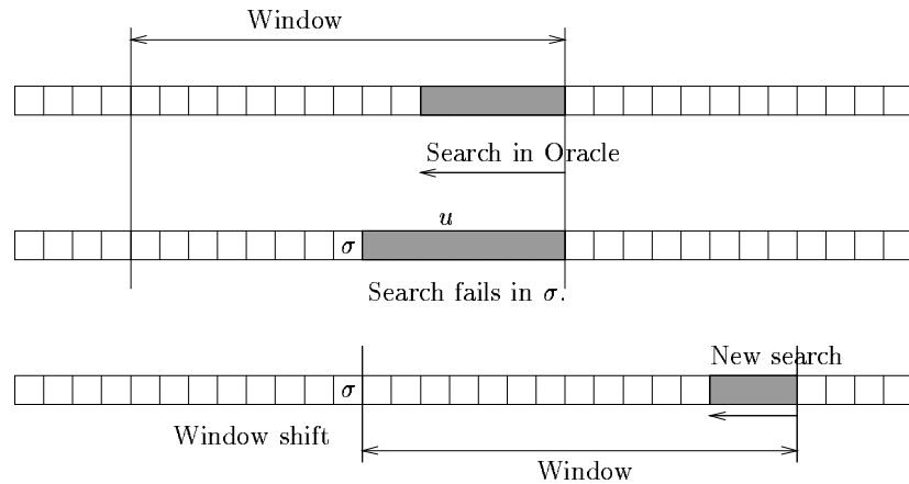
Figure7. Shift of the search window after the fail of the search by Oracle( p ). The word \sigma u is not a factor of p .
